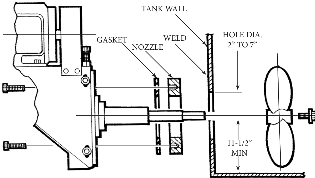
WELD-ON MOUNTING
